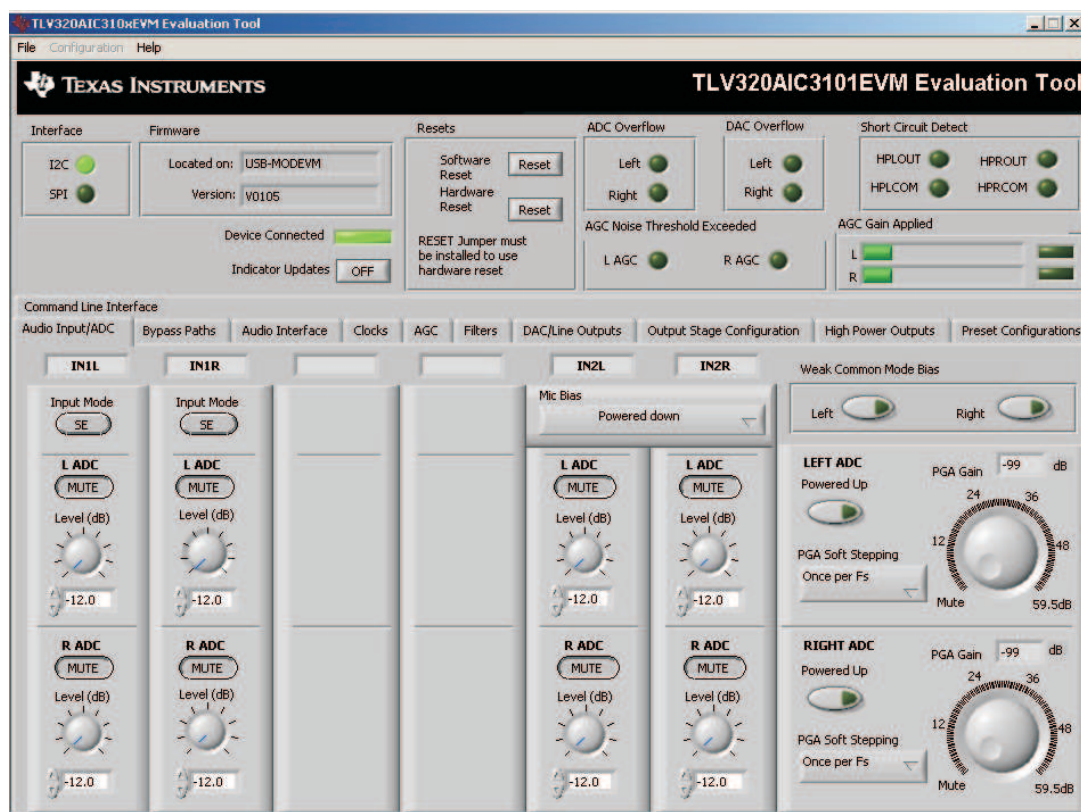
Figure 5. Audio Input/ADC Tab
