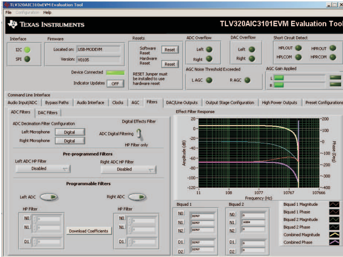
Figure 12. Filters Tab
