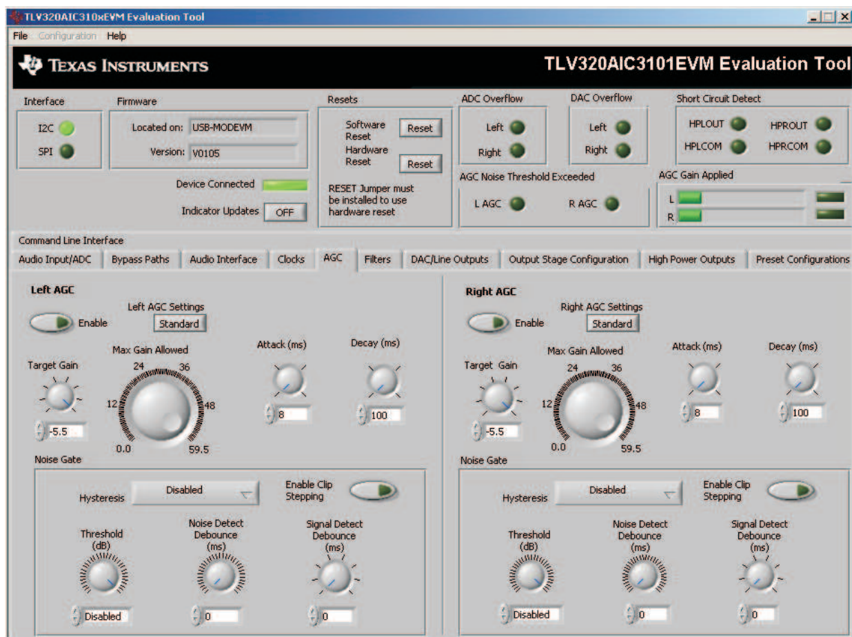
Figure 9. AGC Tab
