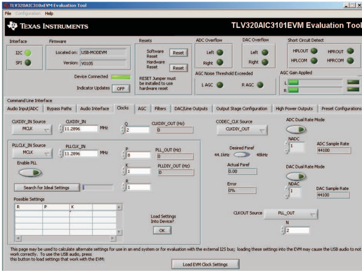
Figure 8. Clocks Tab
